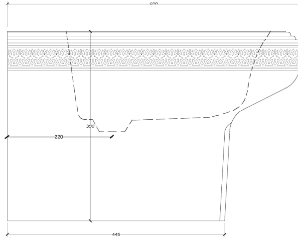
Side Elevation of Bidet
