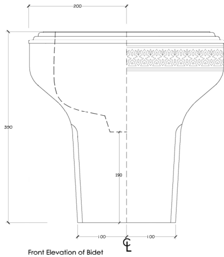
Front Elevation of Bidet
