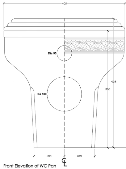
Front Elevation of WC Pan
