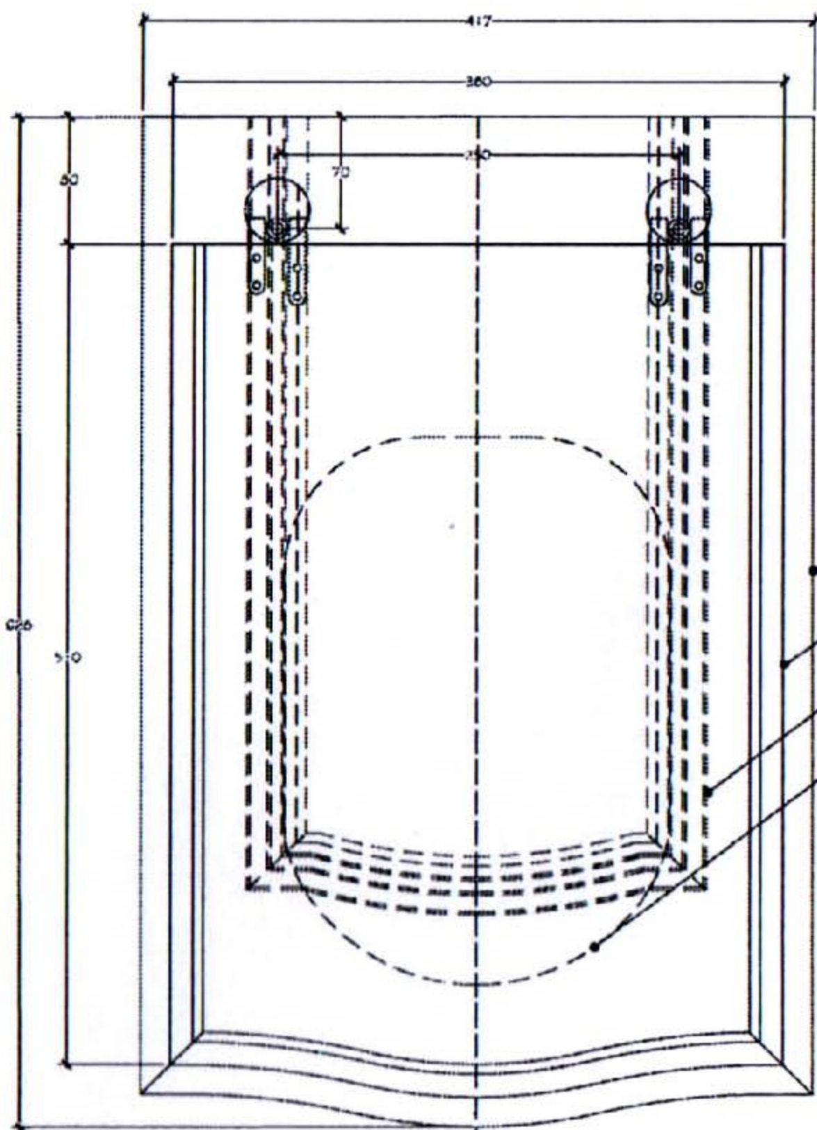
Plan of WC Pan Lid
